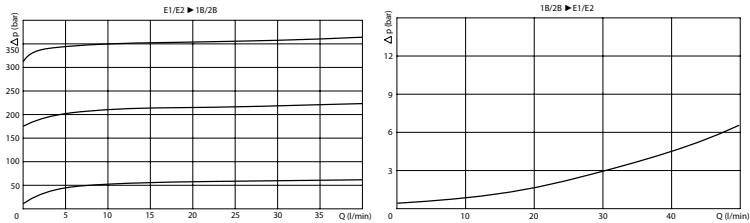
PRESSURE DROP CURVES
